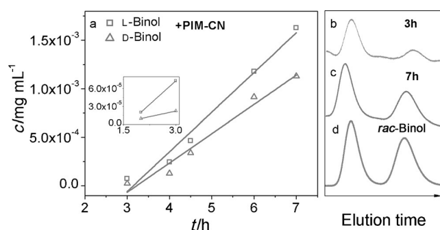
Figure 4. Enantioselective permeation of ( R,S )-binol through (+)-PIM-CN. The inset shows the results at an early stage of permeation. b,c) HPLC chromatogram of the receiver side at 3 and 7 h, respectively, after the start of permeation. d) HPLC chromatogram of racemic binol.
